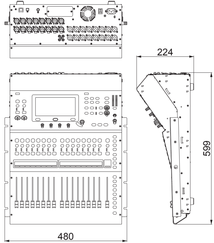
TF1 rack mount (14U)
